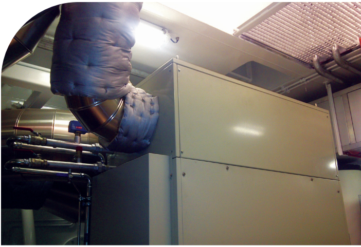
Two liquid natural-gas fueled Capstone C30 MicroTurbines onboard the MTS Argonon Type C tanker in Rotterdam, Netherlands, operate in an N+1 setting and serve as the main electrical power supply.
